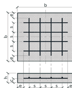
Figure 1 Rebar layout
